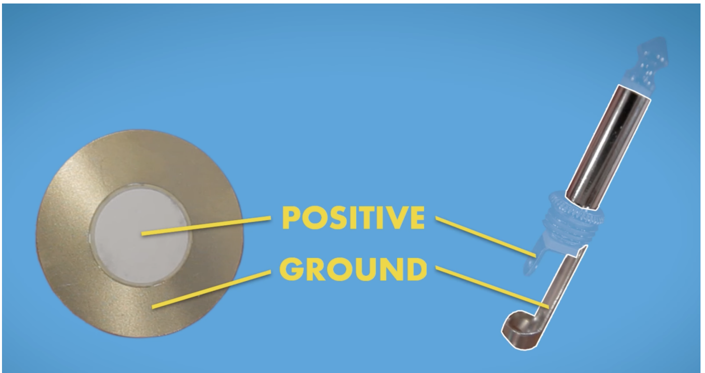
Diagram for balanced wiring
